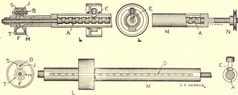
Fig. 89. Traverse Grinder.
